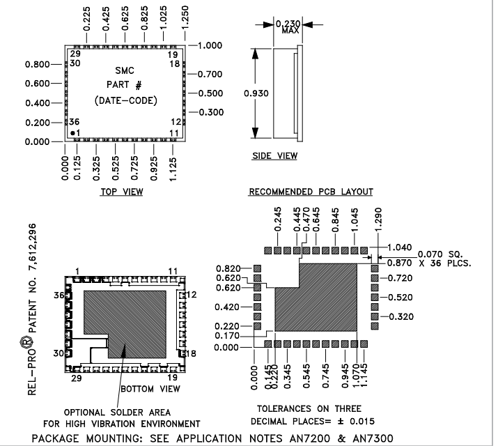
Package # 197LF
