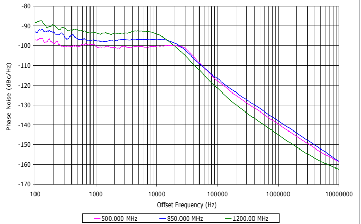
Phase Noise
